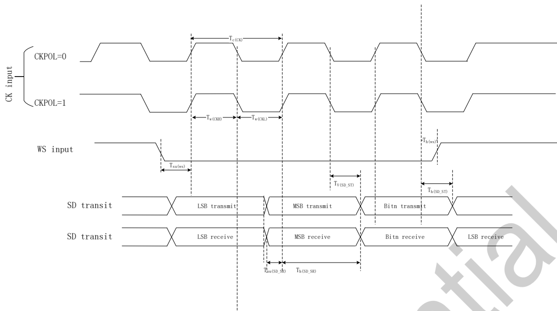
Figure 5-7 I 2 S timing diagram-Slave mode(Philips protocol)
