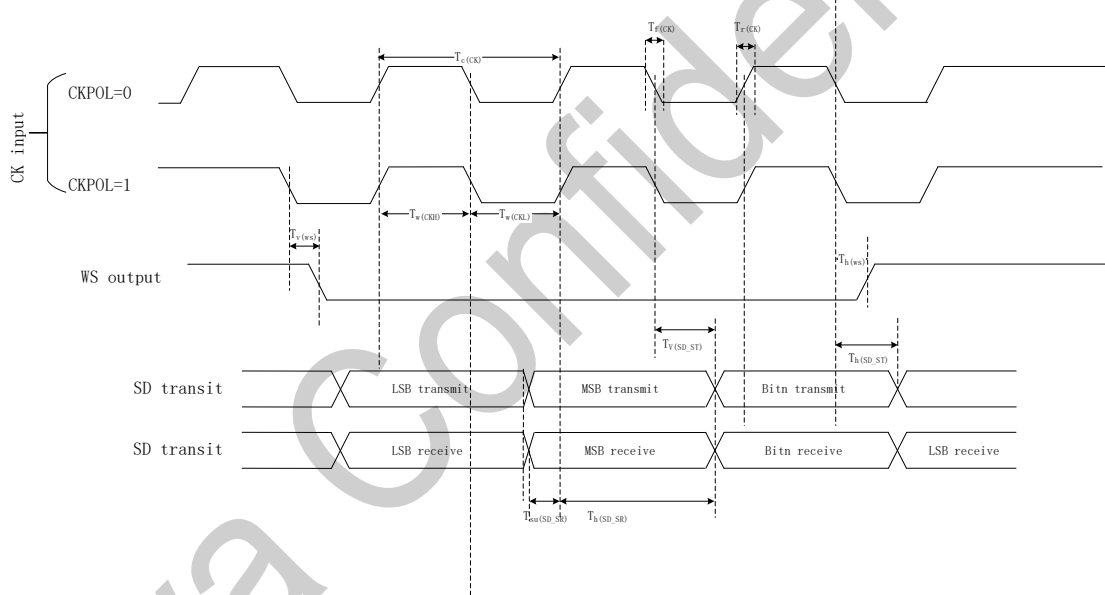
Figure 5-8 I 2 S timing diagram-Master mode(Philips protocol)
